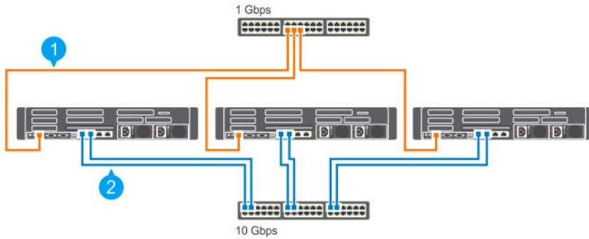
Figure 4. Cabling a system
